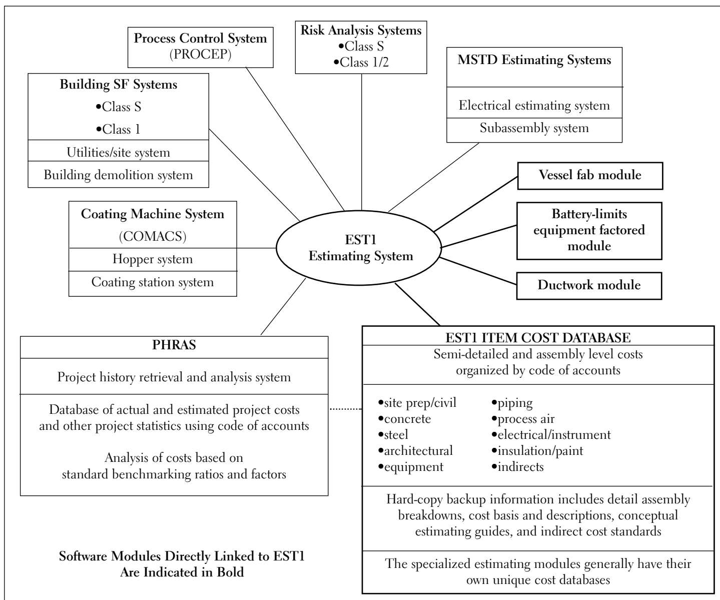
Figure 2—Cost Estimating Systems Diagram
